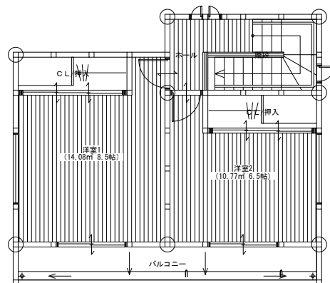
2F(36.44 m 2 )
