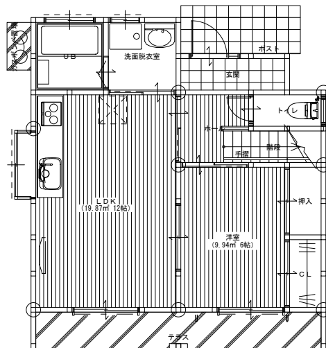
1F(48.86 m 2 )
